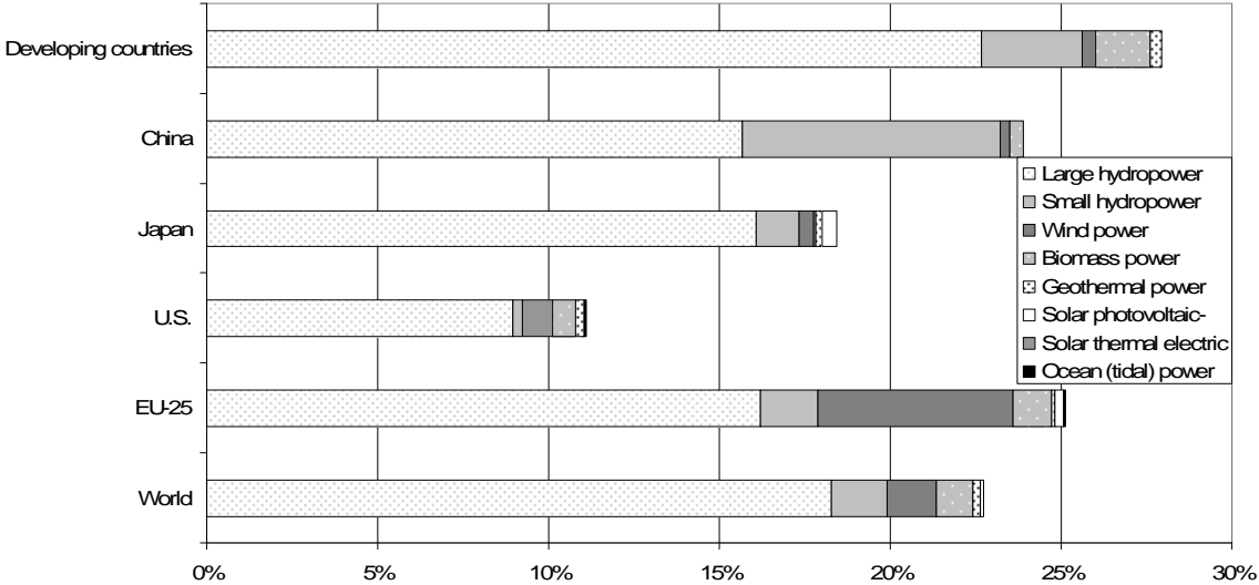
Figure 7. Contribution of Renewable Energy Sources to Total Electricity Supply
