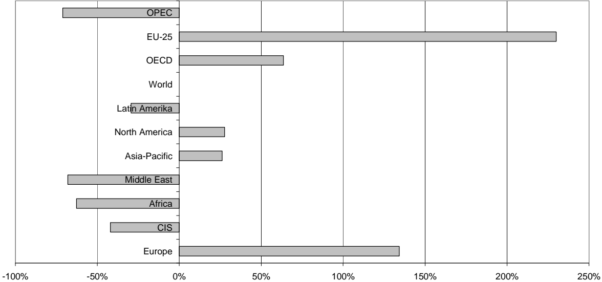
Figure 5. Ratio of Foreign to Domestically Produced Non-Renewable Energy in Main Regions of the World in 2005.
